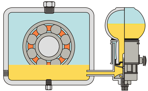
Figure 3. Constant Level Oiler Application.
