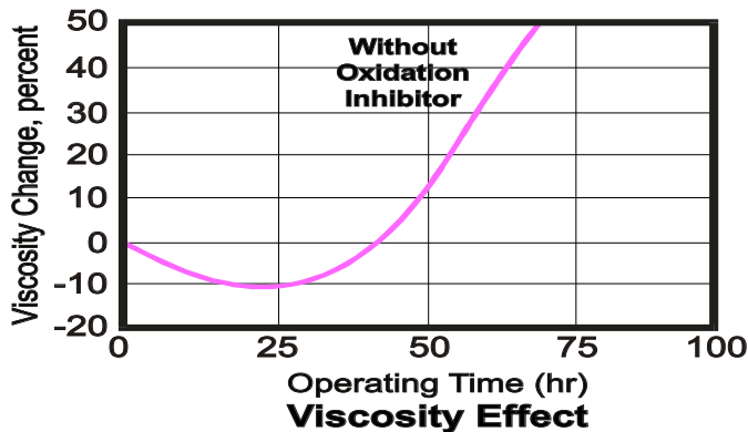
Figure 7. Viscosity Effect as Indicator.
