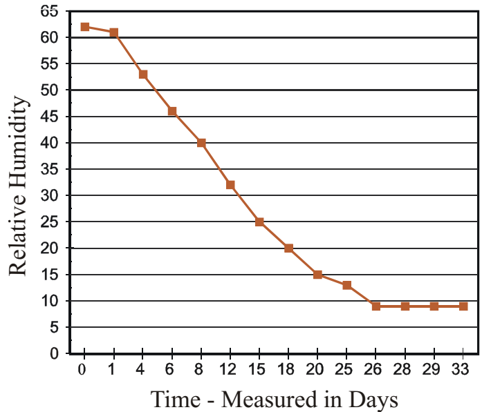
Figure 14. Desiccant Oil Dryer Performance.
