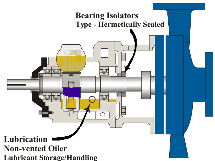
Figure 8. Contamination Ingression Sources
