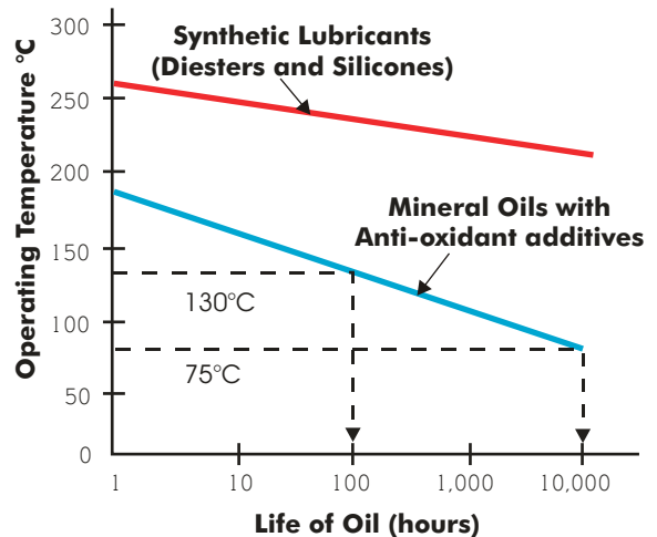
Figure 6. Oil Life Varies with Base Oil Type.
