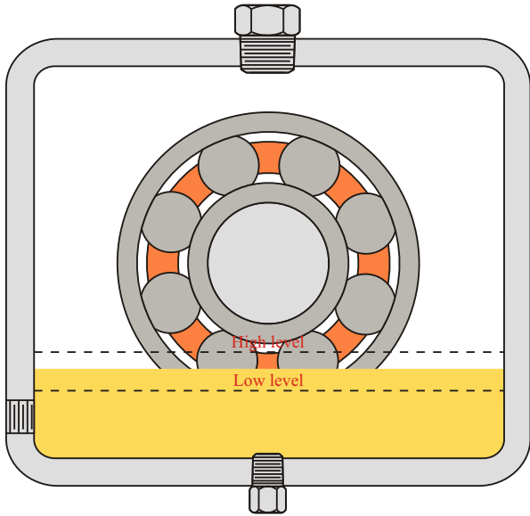
Figure 1. Oil Level Range in Bearing Housing.
