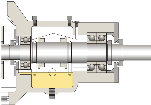
Figure 2. Oil Ring Lubrication.
