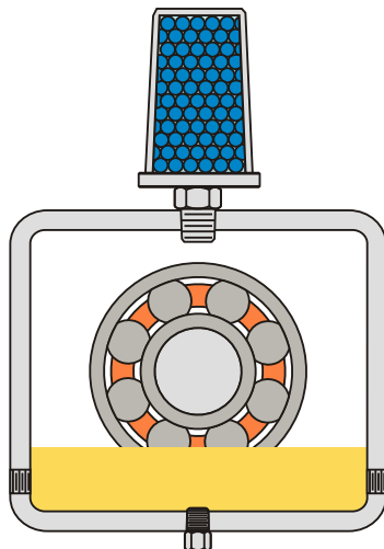
Figure 13. Desiccant Oil Dryer on Bearing Housing.
